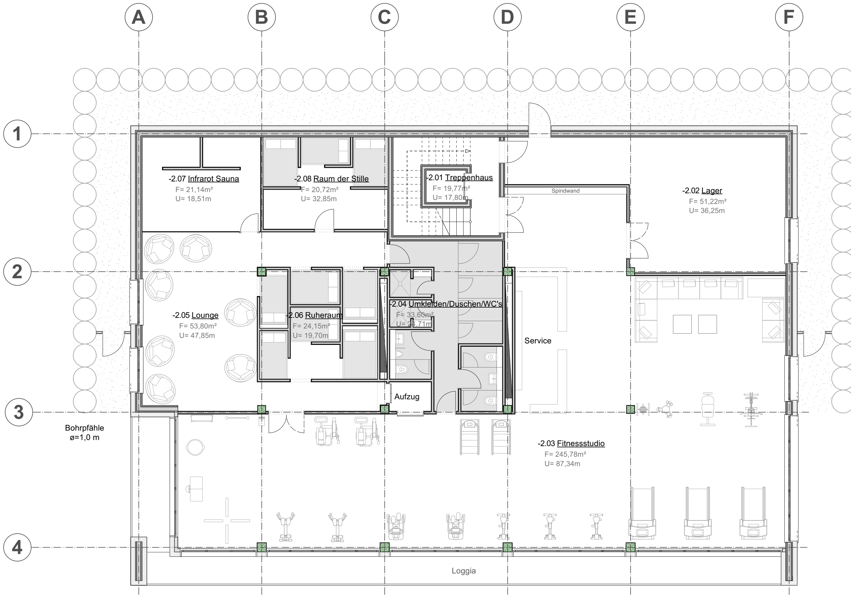
Grundriss Basement 2
