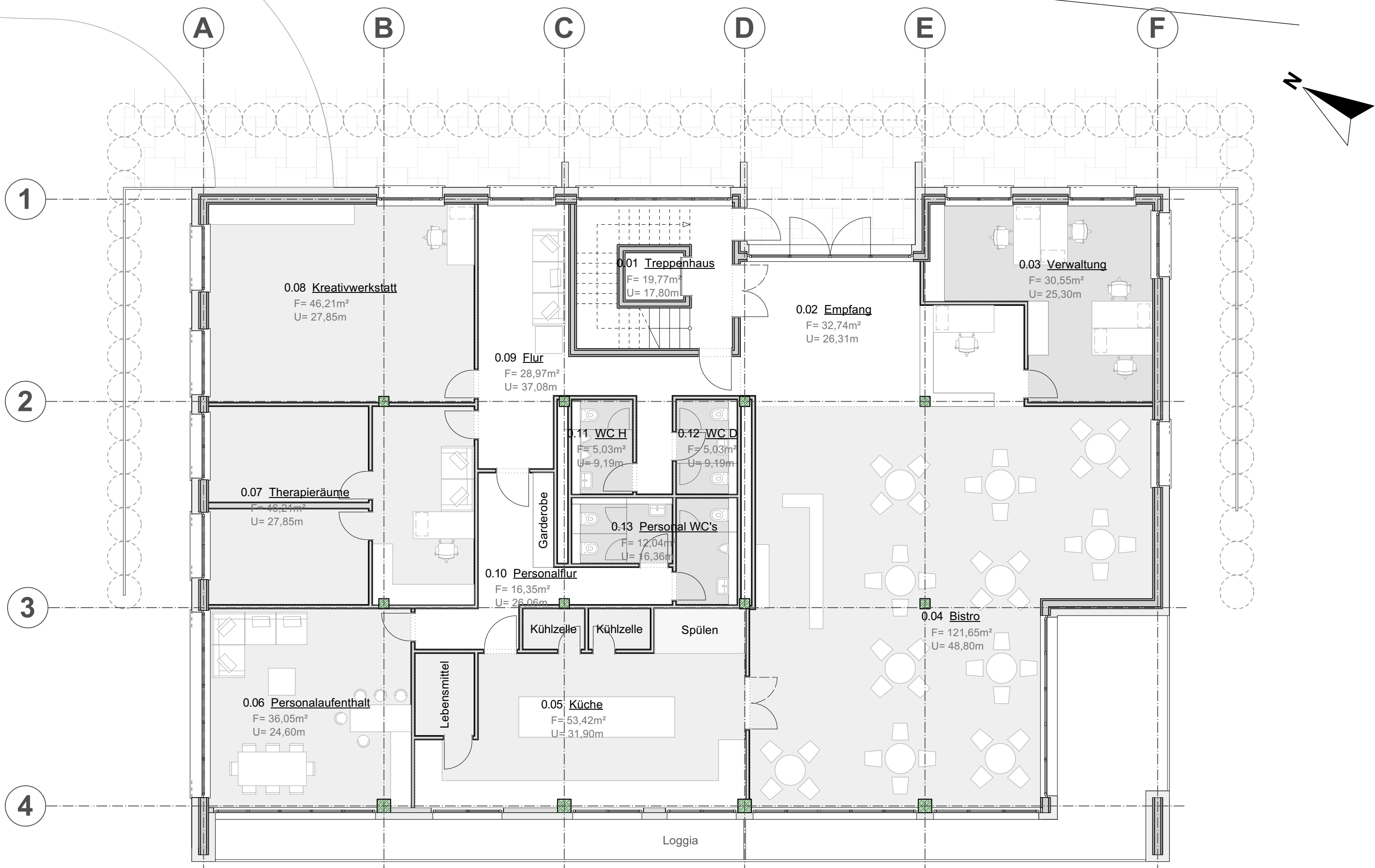
Grundriss Lobby/Restauration
